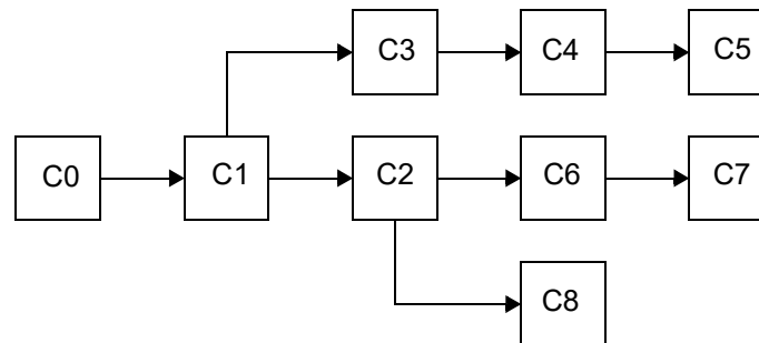
Figure 28 Example of Pulling Cells in a Contiguous Datapath
