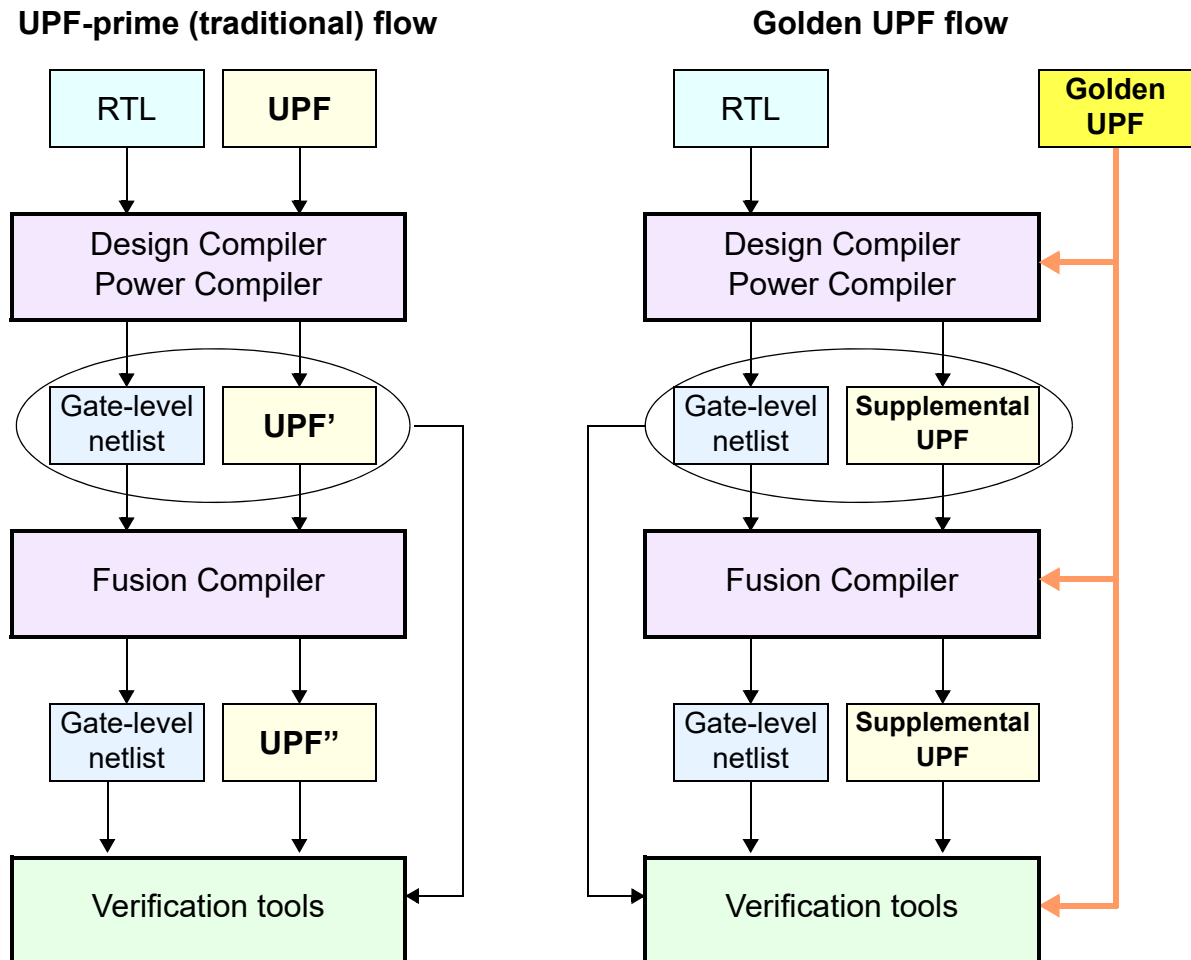
Figure 3 UPF-Prime (Traditional) and Golden UPF Flows
