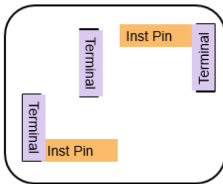
Figure 72 Layout With Power and Ground Terminals
