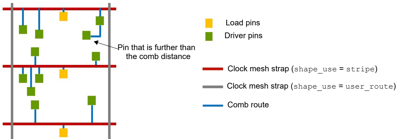
Figure 47 Comb Topology
