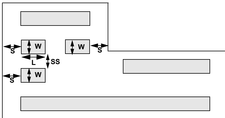
Figure 55 Metal Shape Perimeter Constraint Objects With Additional Short Shapes
