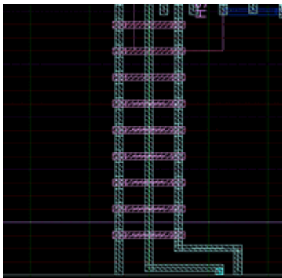
Figure 68 Coaxial Shielding
