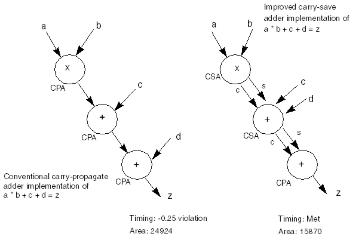
Figure 2 Conventional Carry-Propagate Adder Versus Carry-Save Adder
