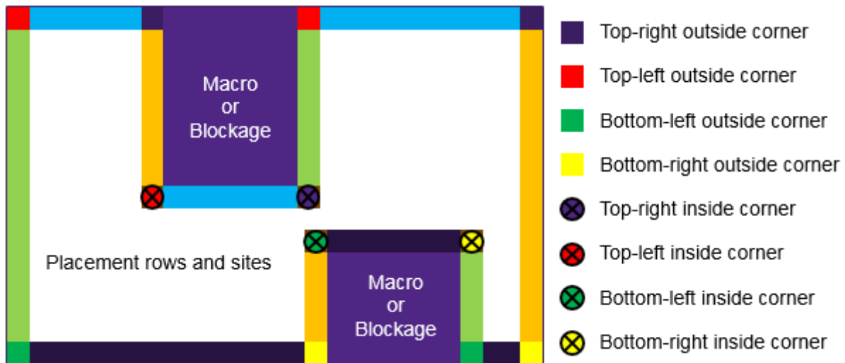
Figure 75 Boundary Cell Locations
