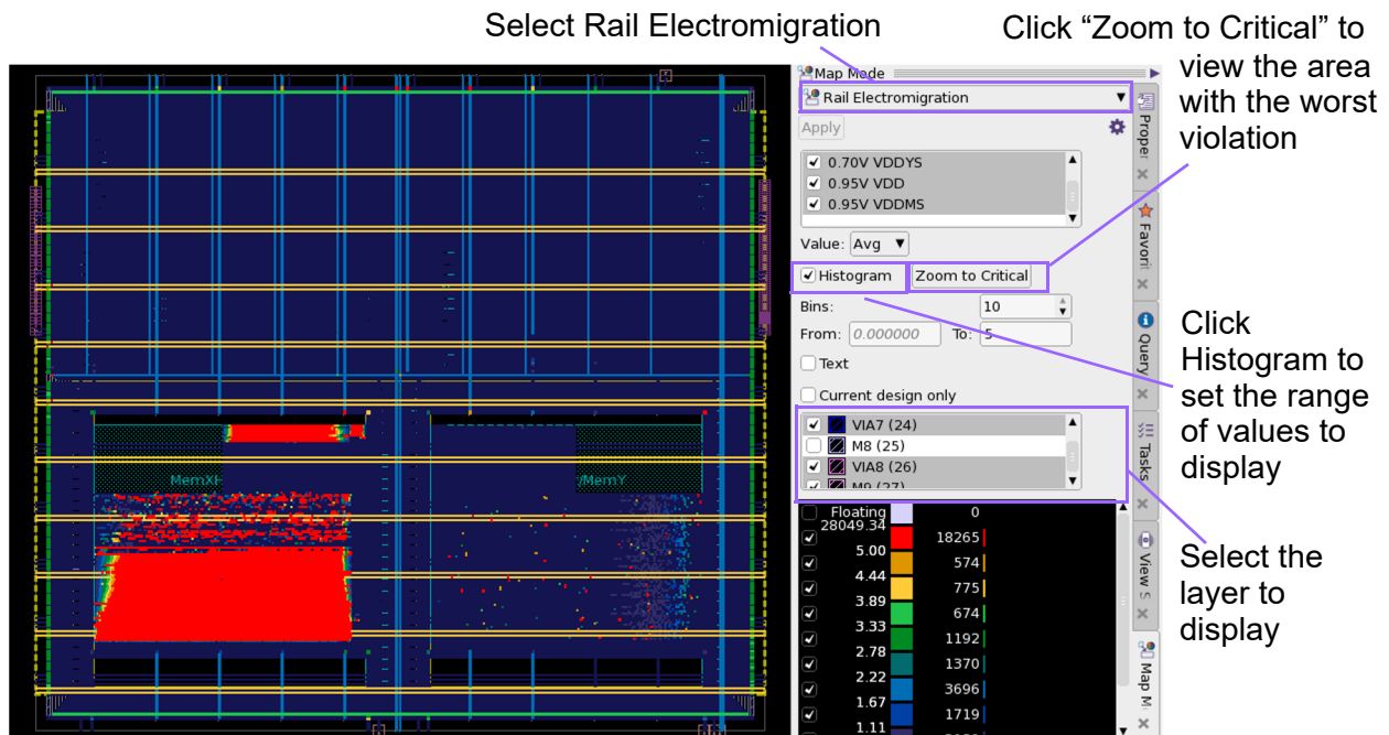
Figure 127 Displaying a PG Electromigration Map
