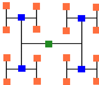
Figure 41 Clock Drivers Placed in an H-Tree Structure
