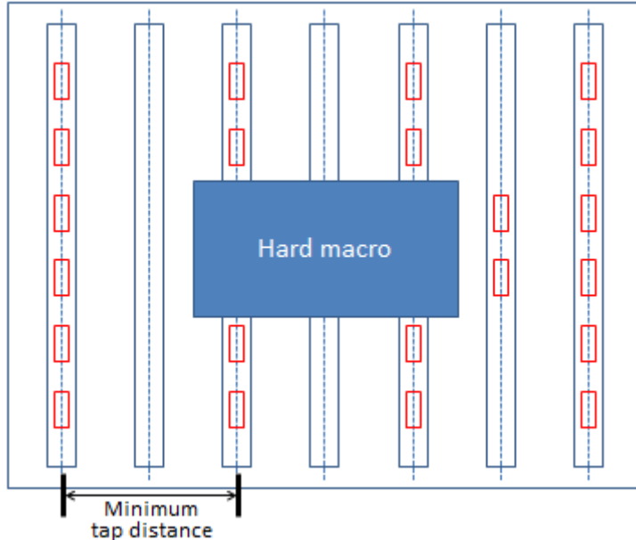
Figure 73 Default Tap Cell Placement
