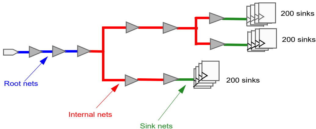
Figure 59 Root, Internal, and Sink Clock Net Types
