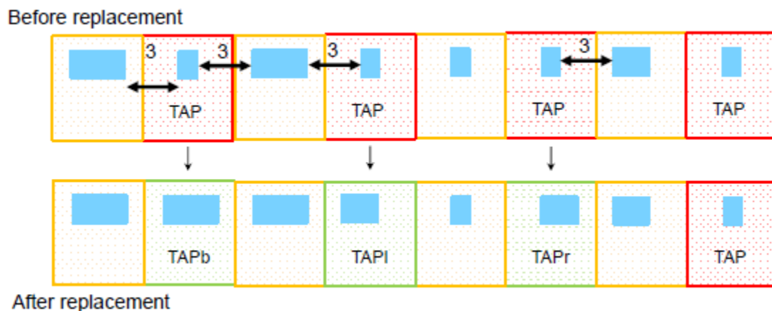
Figure 86 Fixing a Tap Cell Spacing Violation
