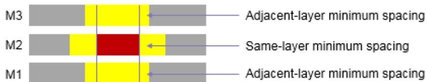
Figure 88 Minimum Spacing From Metal Fill to Critical Net Shape
