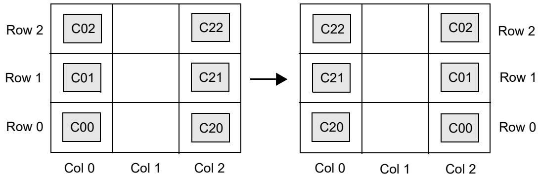
Figure 109 Swapping Columns of a Relative Placement Group
