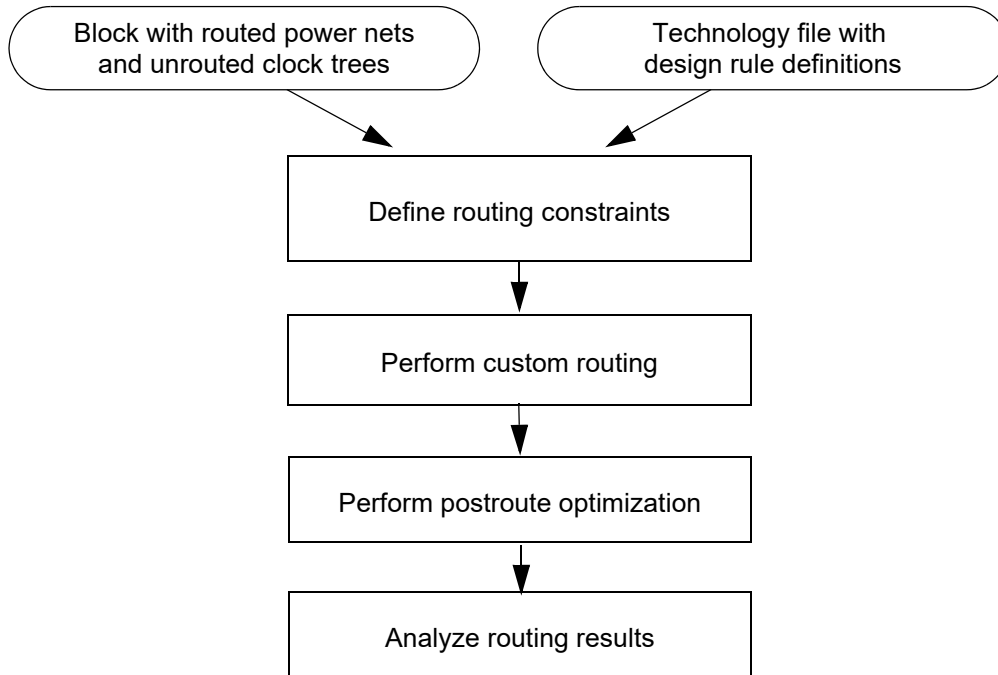
Figure 90 Basic Custom Router Flow
