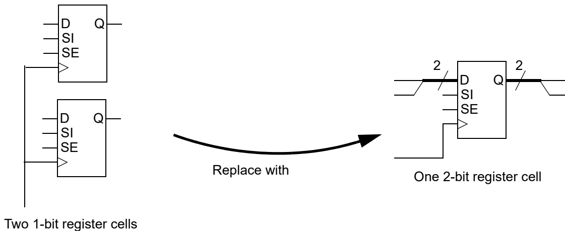
Figure 5 Replacing Multiple Single-Bit Register Cells With a Multibit Register Cell
