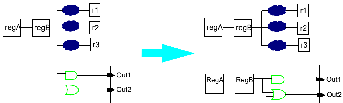
Figure 3 Before and After Register Replication
