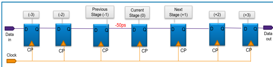
Figure 37 Previous, Current, and Next Path Stages
