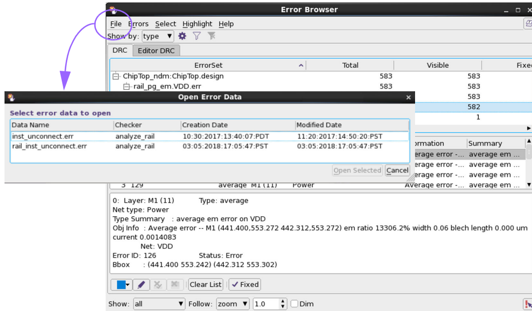
Figure 125 Opening Error Data from the Error Browser
