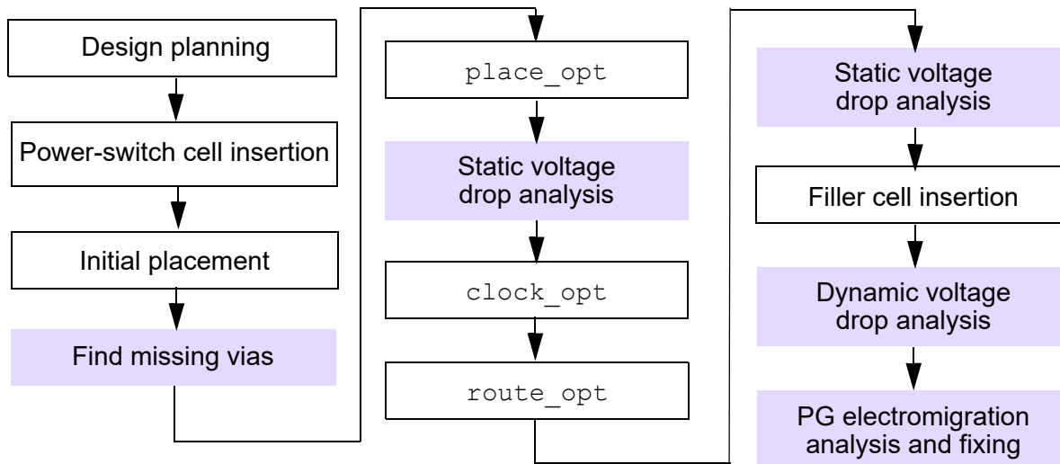
Figure 121 Using RedHawk Analysis Fusion in the Fusion Compiler Design Flow
