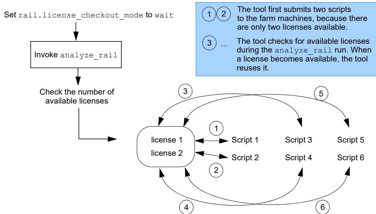
Figure 131 Waiting for Available Licenses During Distributed RedHawk Analysis Fusion Run
