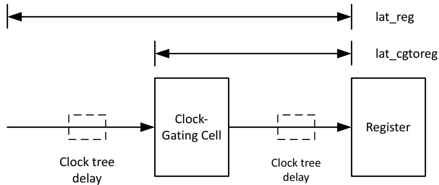
Figure 9 Clock Latency With Clock-Gating Design
