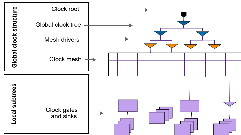
Figure 39 Structural Multisource Clock Tree
