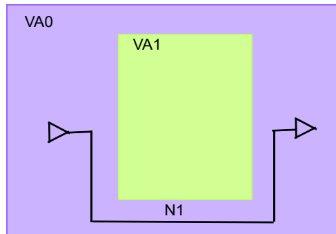
Figure 26 Physical-Feedthrough Nets Disabled for a Voltage Area
