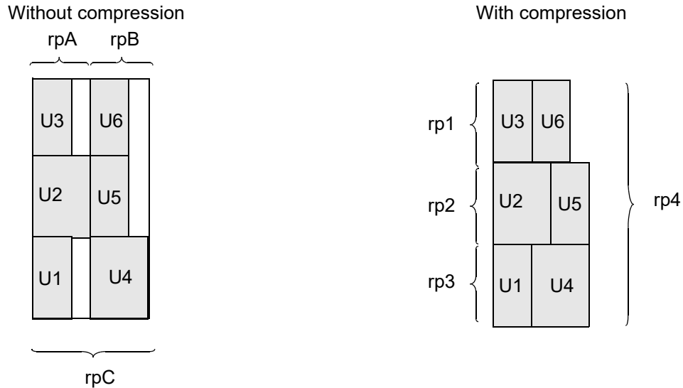
Figure 97 Bottom-Left Alignment Construction and Compression
