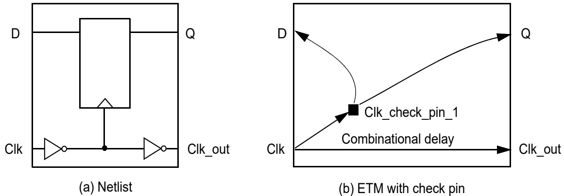
Figure 34 Module With Combinational Clock Path
