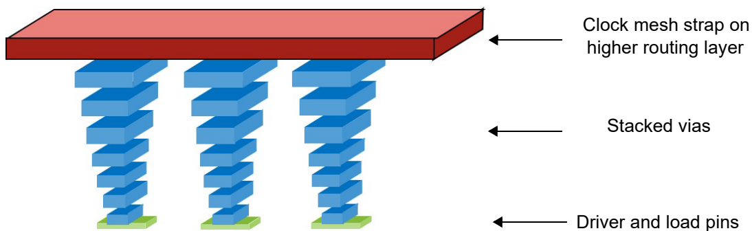
Figure 48 Vias in the Comb Topology
