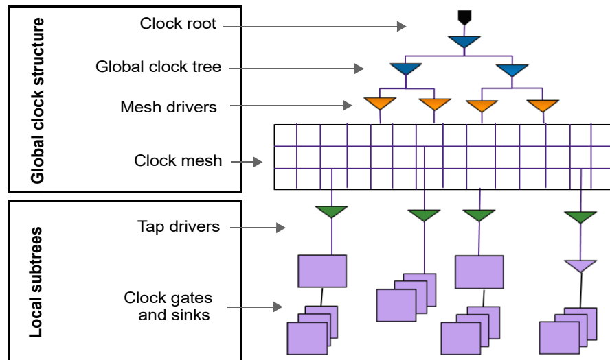
Figure 38 Regular Multisource Clock Tree
