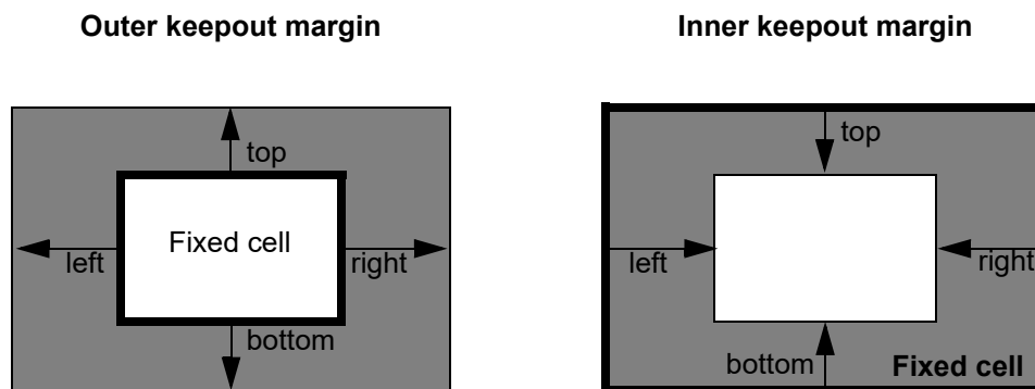
Figure 19 Placement Keepout Margins
