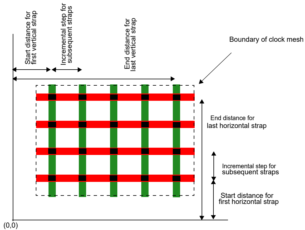
Figure 42 Clock Mesh Structure
