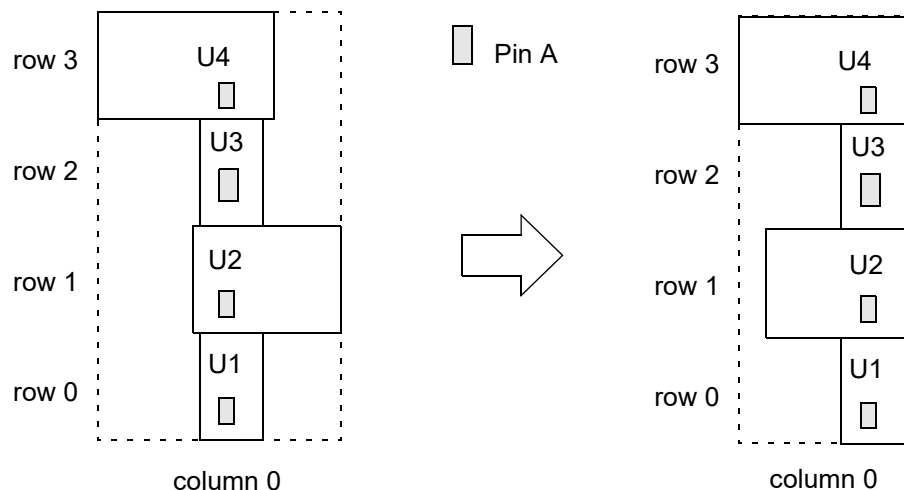
Figure 103 Minimizing the Column Width of a Relative Placement Group Aligned by Pins
