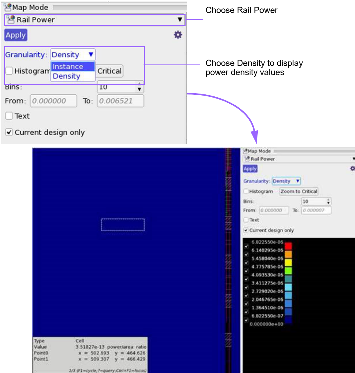
Figure 134 Displaying a Power Density Map
