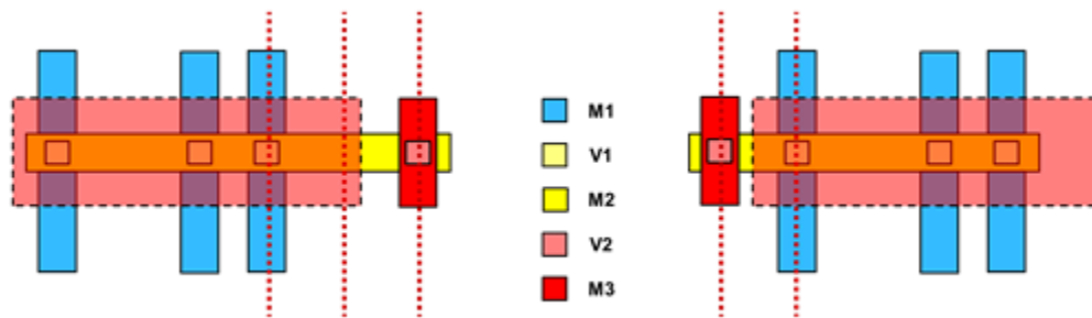
Figure 64 Pattern-Based Must-Join Pin Connection With Staggering
