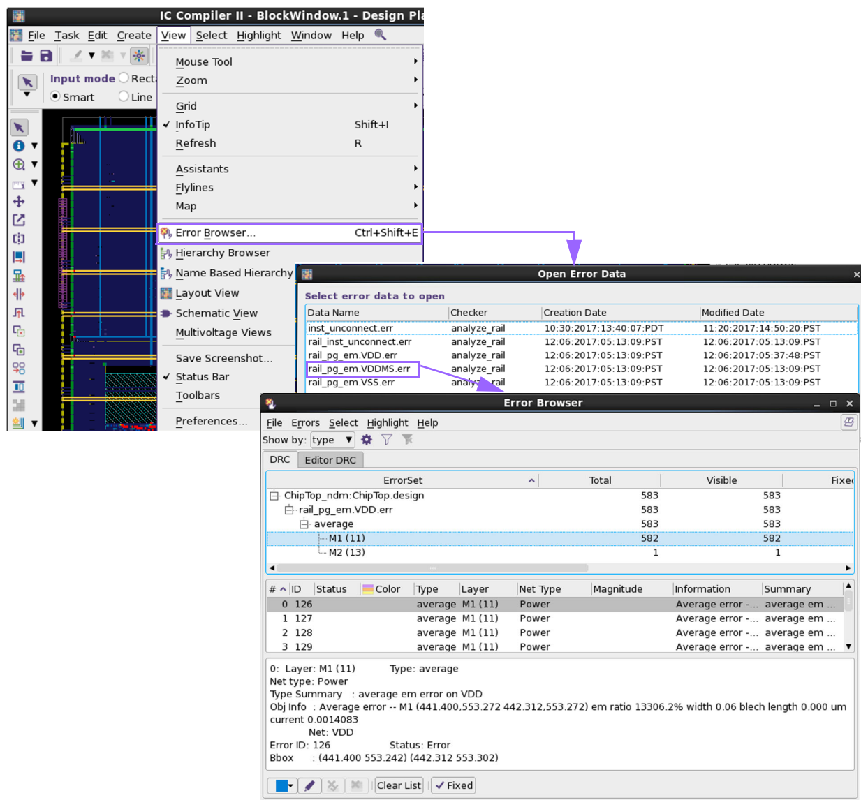
Figure 128 Opening Generated Errors in the Error Browser
