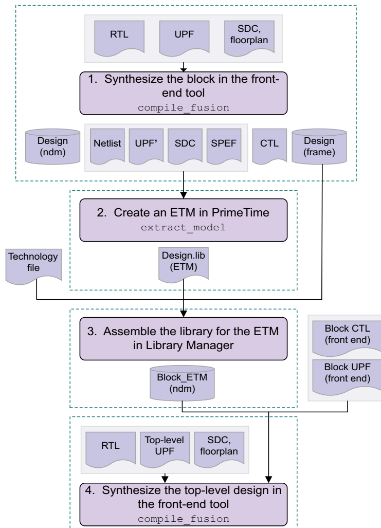
Figure 113 Hierarchical Synthesis Feasibility Analysis
