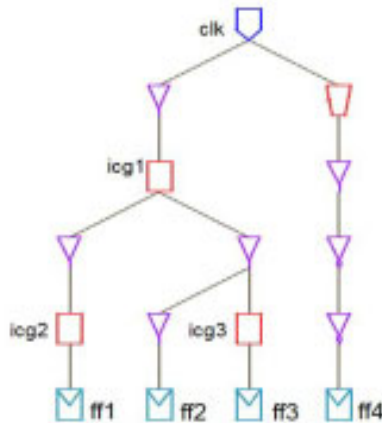
Figure 51 Segments and Subtrees of a Clock Tree
