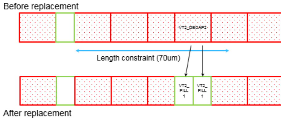
Figure 82 Fixing a Maximum Vertical Edge Length Violation
