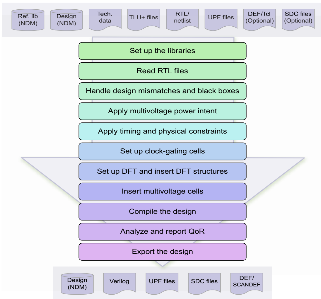
Figure 1 Fusion Compiler Physical Synthesis Flow
