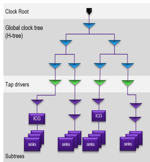
Figure 40 Regular Multisource Clock Tree With an H-Tree-Only Global Clock Structure
