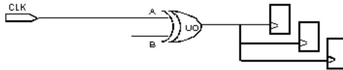
Figure 29 Non-Unate Gated Clock
