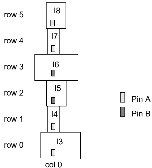
Figure 104 Relative Placement Group Aligned by Different Pins
