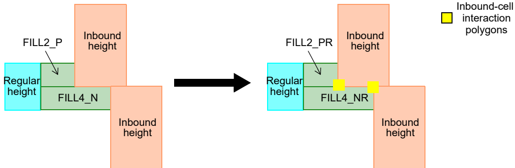
Figure 80 Half-Height Filler Cell Replacement With Half Row Adjacency Rule
