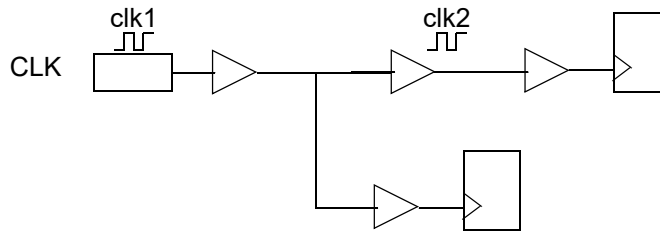
Figure 31 Cascaded Clock With Two Source Clocks
