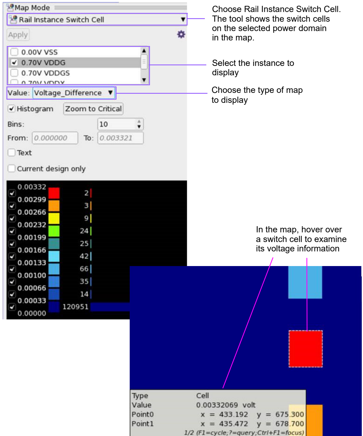
Figure 133 Displaying Maps for Switch Cells
