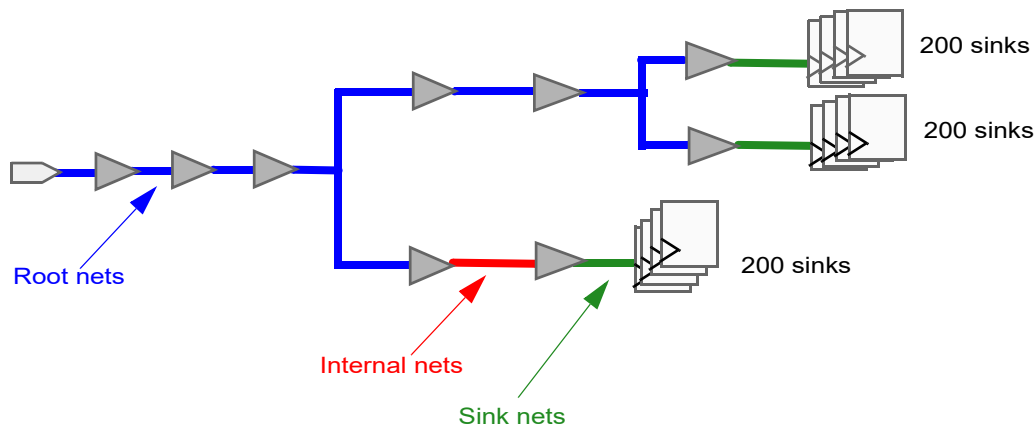
Figure 2 Using a Fanout Limit for Selecting Root Nets
