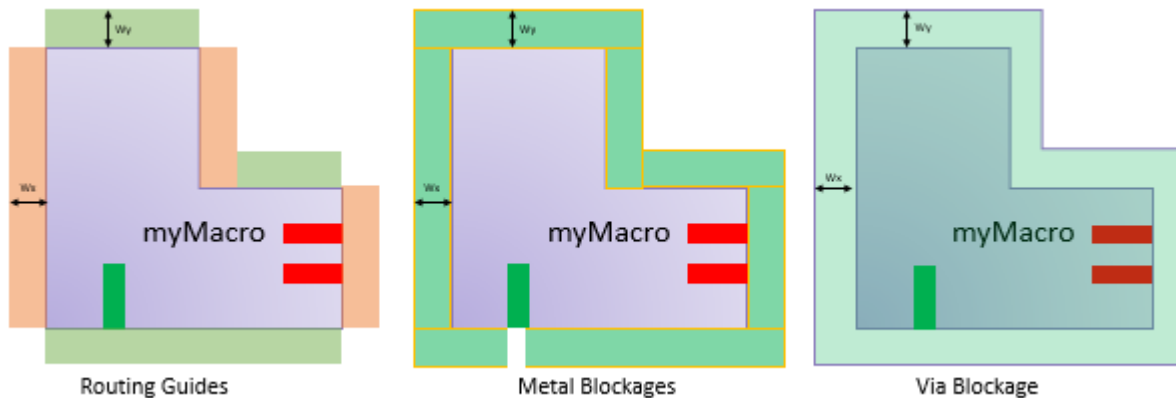
Figure 53 Pin Access Routing Guides and Blockages
