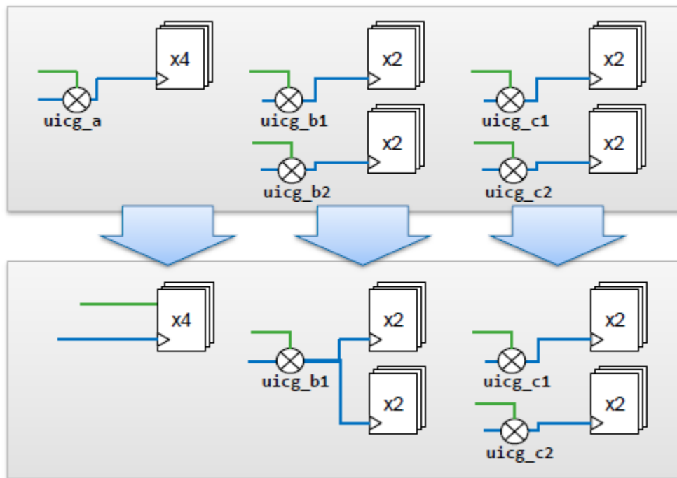
Figure 12 Example of Clock Gating Restrictions
