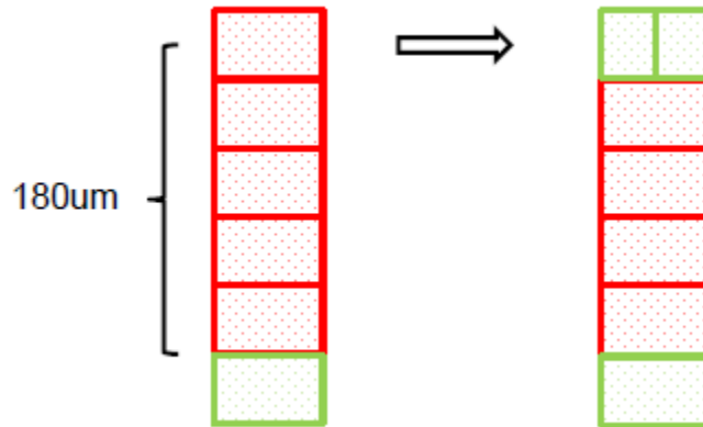
Figure 85 Fixing a Maximum Vertical Edge Length Violation
