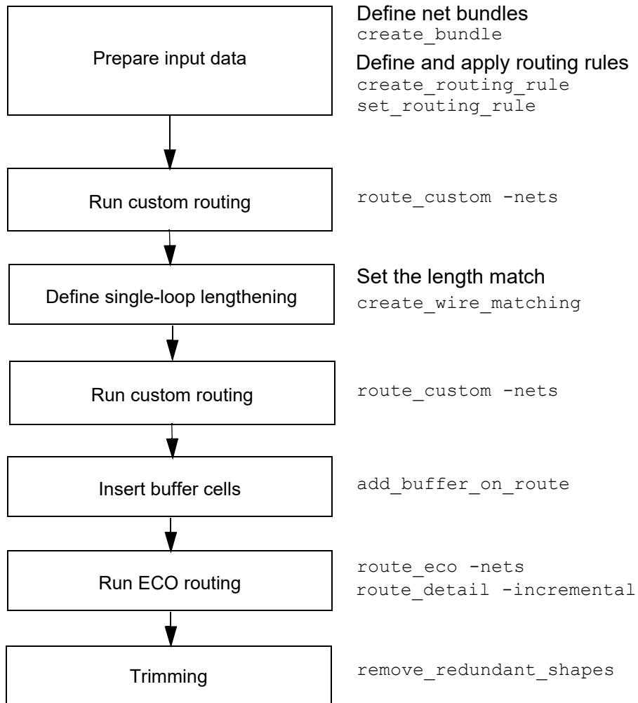
Figure 91 A Basic DDR Flow
