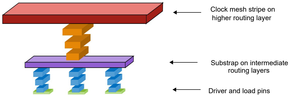
Figure 49 Vias in the Substrap Topology
