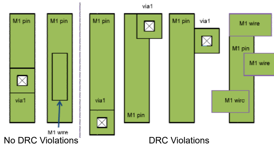
Figure 67 Restricted Via-to-Pin and Wire-to-Pin Connections
