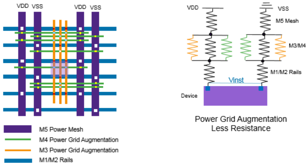
Figure 87 Power Grid Augmentation
