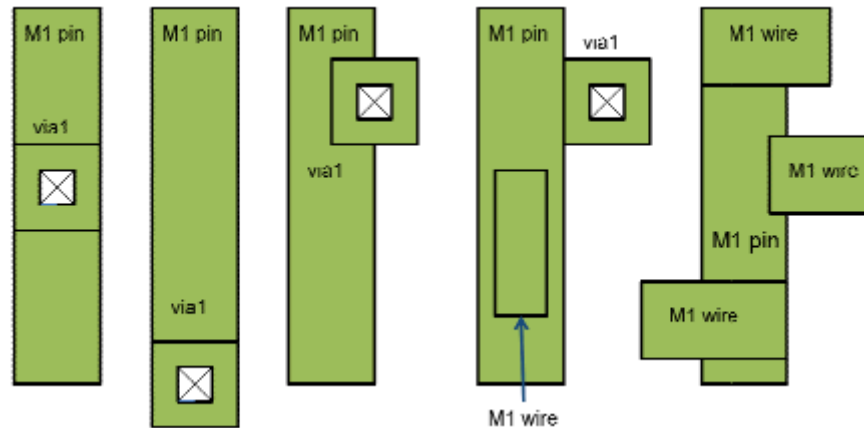
Figure 65 Unrestricted Pin Connections
