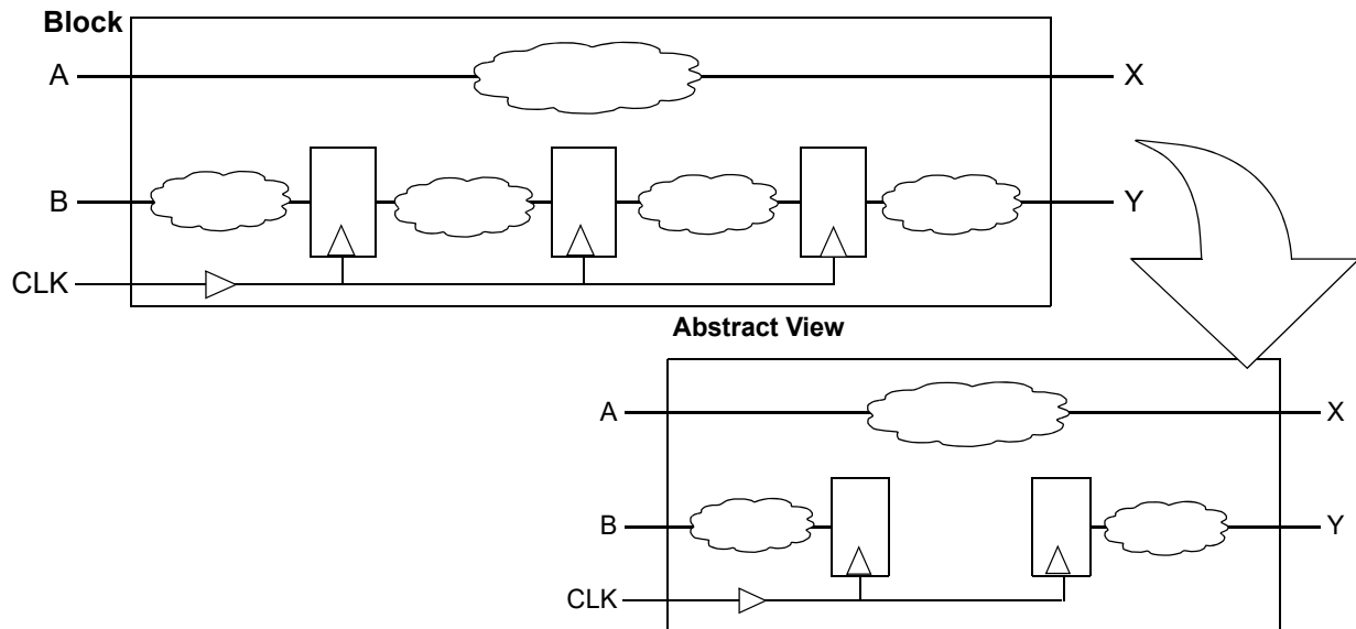
Figure 115 A Block and Its Abstract View
