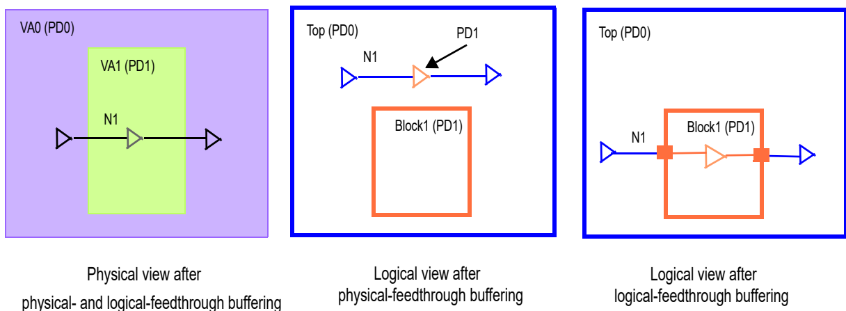
Figure 27 Difference in the Logical View After Physical- and Logical-Feedthrough Buffering
