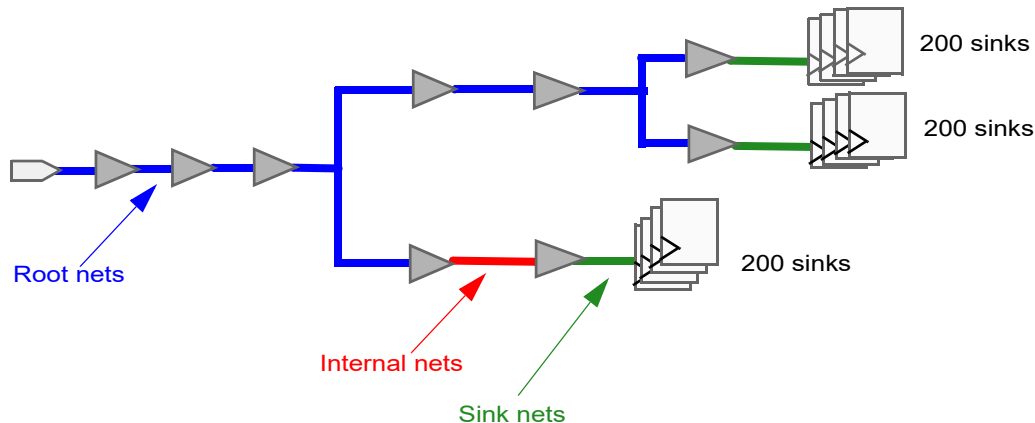
Figure 60 Using a Fanout Limit for Selecting Root Nets
