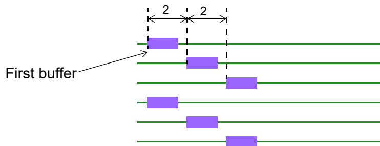
Figure 138 Buffer Patterns for a Horizontal Bus
