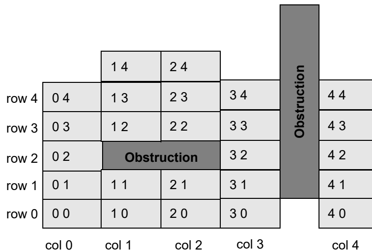
Figure 111 Relative Placement in a Design Containing Obstructions
