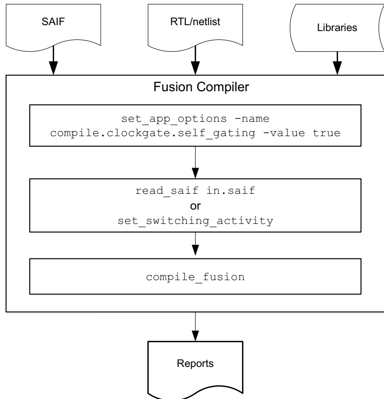
Figure 18 General Self-Gating Flow
