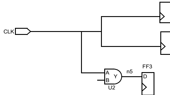
Figure 33 Specifying Exceptions on Pins Beyond the Clock Network
