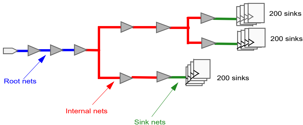
Figure 1 Root, Internal, and Sink Clock Net Types
