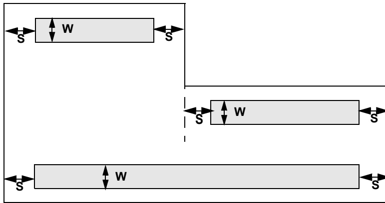
Figure 54 Metal Shape Perimeter Constraint Objects
