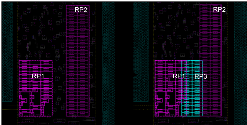
Figure 112 Legalizing the RP3 Relative Placement Group Over Other Groups
