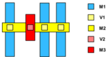
Figure 63 Multi-Level Pattern-Based Must-Join Pin Connection
