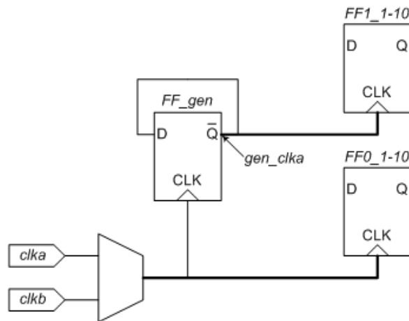
Figure 35 Clock Pins That Cannot Be Balanced Simultaneously
