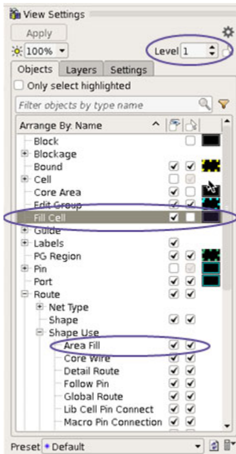
Figure 89 Settings Used to Display Fill Shapes in the GUI
