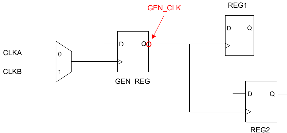
Figure 36 Generated Clock With Invalid Master Clock Source
