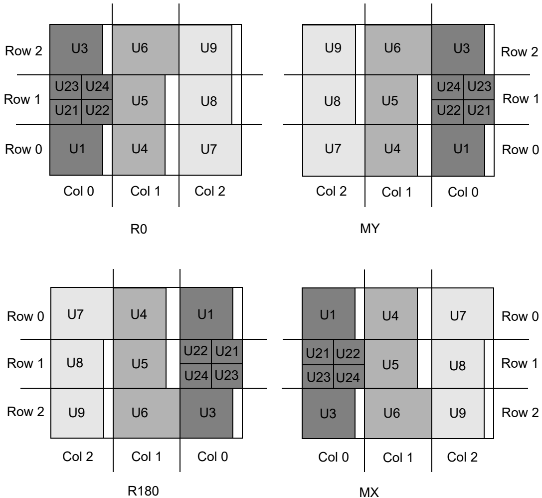
Figure 108 Orientation of Relative Placement Groups
