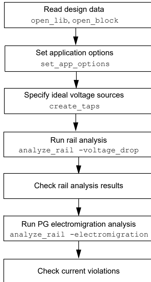
Figure 123 Required Steps for a Basic Rail Analysis Using RedHawk Analysis Fusion
