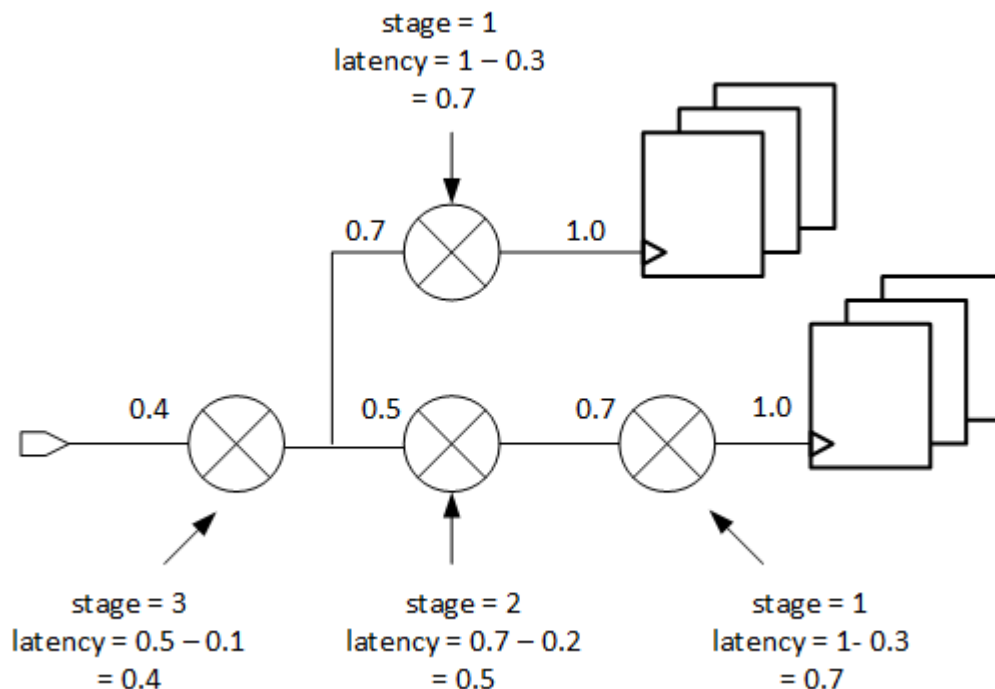
Figure 10 Clock-Gating Stages and Latency Calculations
