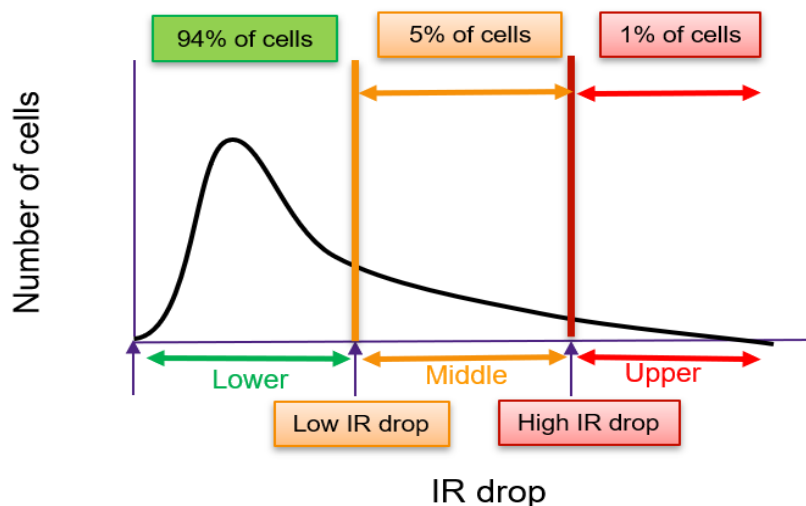
Figure 20 Default Cell Categories for IR-Drop-Aware Placement
