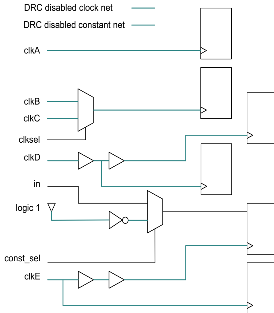
Figure 6 DRC Disabled Clock and Constant Nets Highlighted
