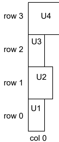
Figure 101 Bottom-Left-Aligned Relative Placement Group
