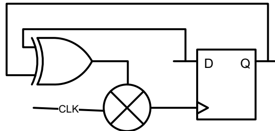
Figure 16 Example of a Self-Gating Cell
