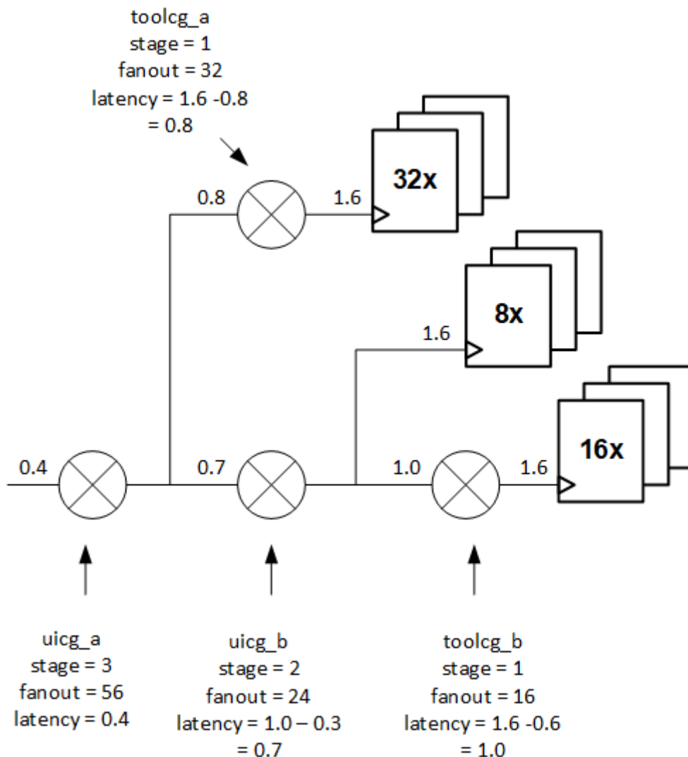
Figure 11 Latency Calculations with Varying Fanout
