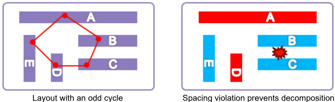
Figure 5 Odd-Cycle Violation
