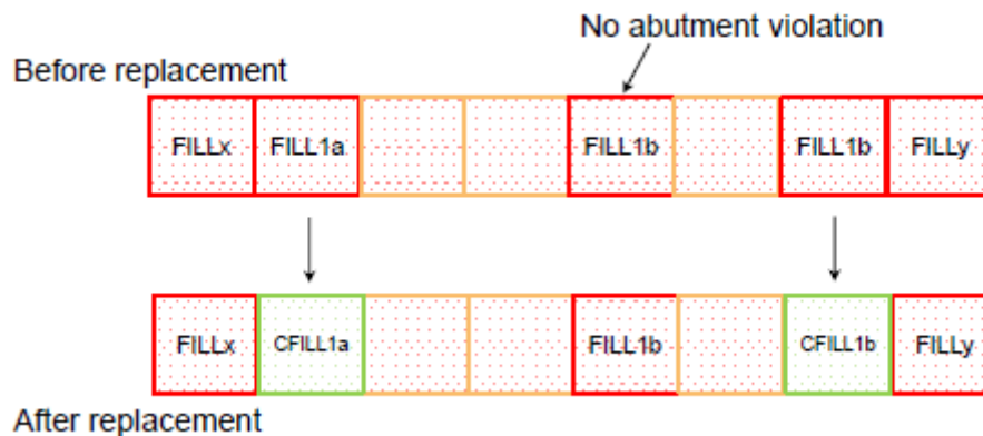
Figure 81 Fixing an Illegal Abutment Violation
