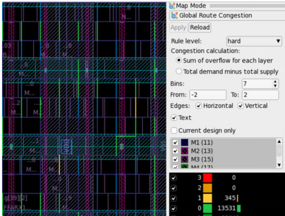
Figure 70 Global Route Congestion Map
