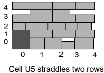
Figure 107 Compression of a Relative Placement Group With a Cell That Straddles Multiple Rows
