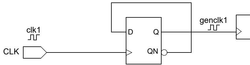
Figure 30 Nested Clock Tree With a Generated Clock
