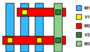
Figure 61 Default Must-Join Pin Connection
