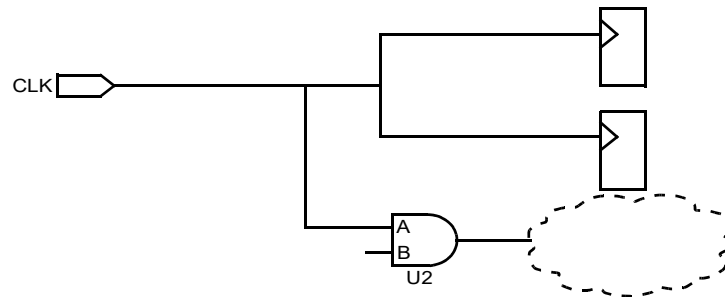
Figure 32 User-Defined Ignore Pin
