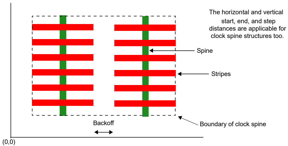
Figure 43 Clock Spine Structure
