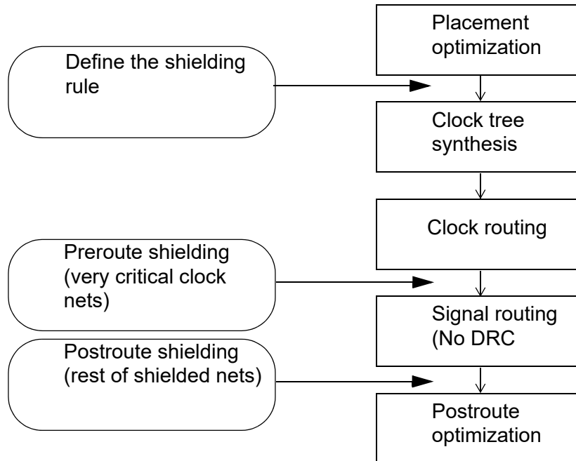
Figure 69 Zroute Shielding Flow
