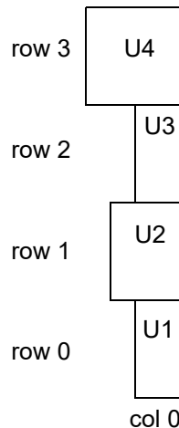
Figure 102 Bottom-Right-Aligned Relative Placement Group
