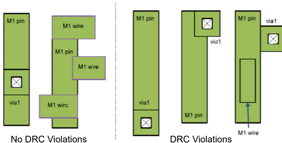
Figure 66 Restricted Via-to-Pin Connections
