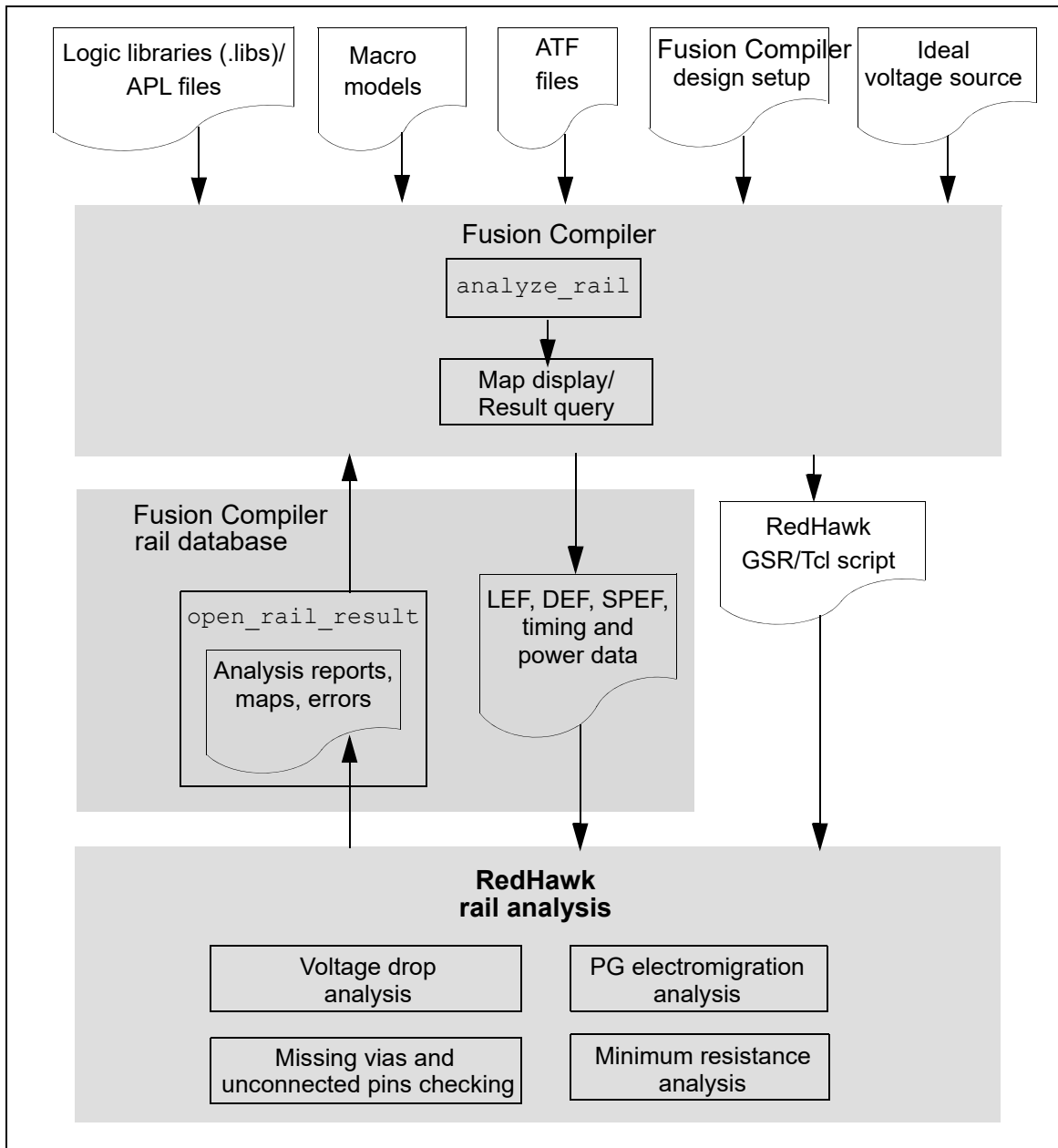
Figure 122 RedHawk Analysis Fusion Data Flow
