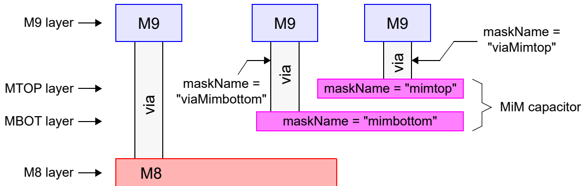
Figure 79 Cross-Section View of MiM Capacitor Layers
