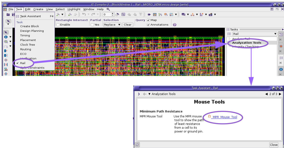
Figure 129 Invoking the MPR Mouse Tool
