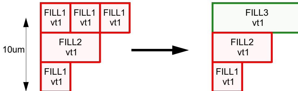
Figure 83 Fixing Maximum Stacking Violation by Replacement
