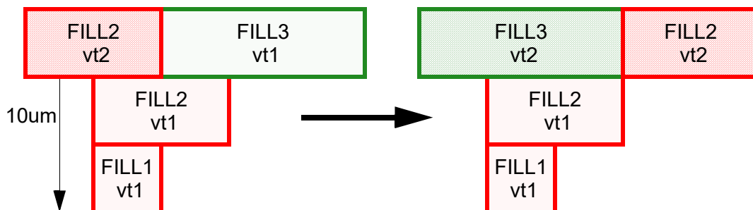
Figure 84 Fixing Maximum Stacking Violation by Reordering
