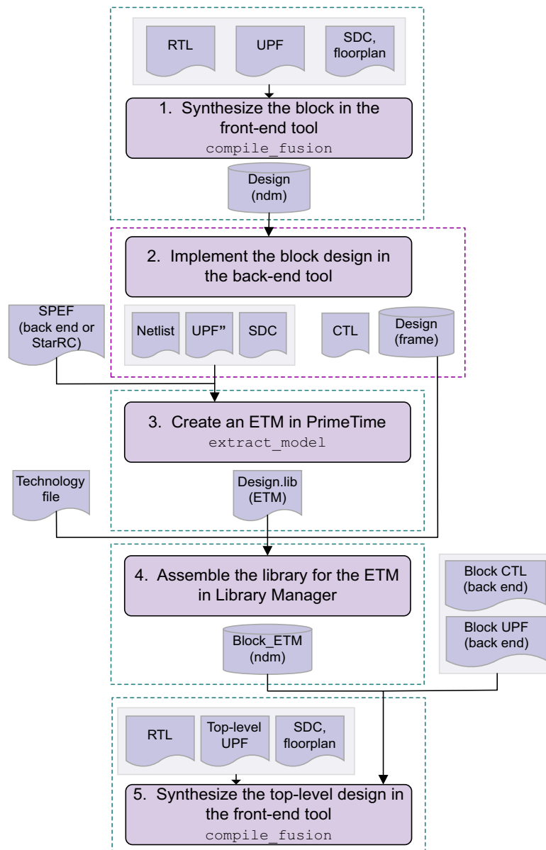
Figure 114 Hierarchical Synthesis Flow
