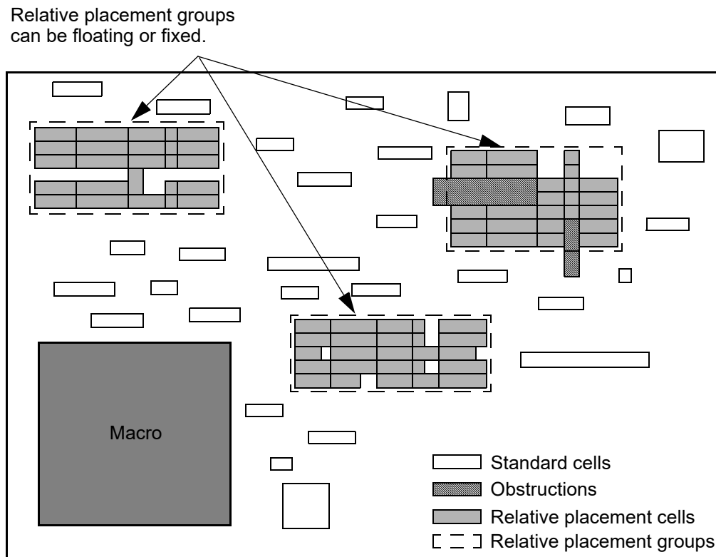
Figure 92 Relative Placement in a Floorplan
