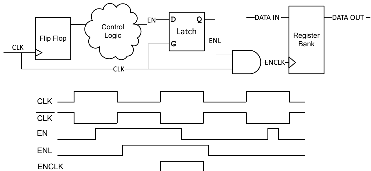
Figure 8 Latch-Based Clock Gating
