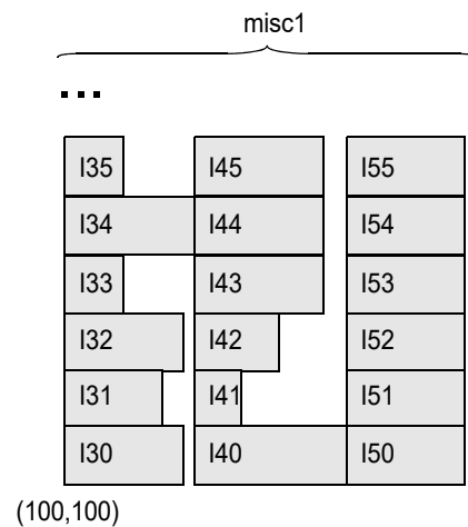
Figure 99 Anchored Relative Placement Group
