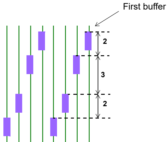
Figure 139 Buffer Patterns for a Vertical Bus
