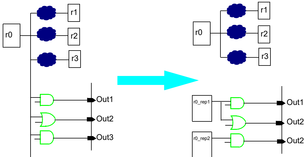
Figure 4 Using the -driven_by_original_register Option
