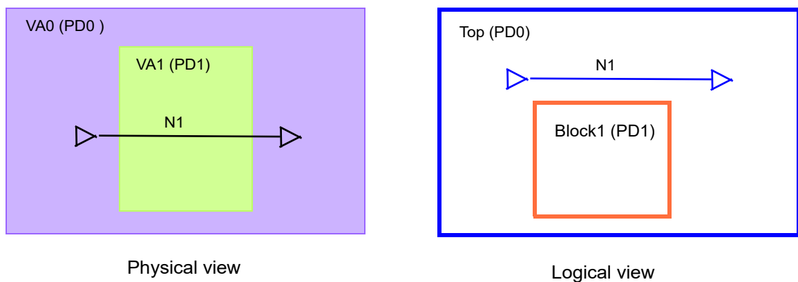
Figure 25 Physical-Feedthrough Nets of Voltage Areas
