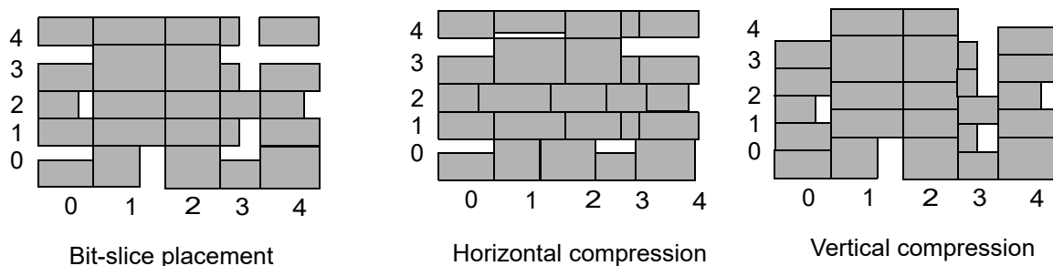
Figure 106 Bit-Slice Placement Versus Horizontal or Vertical Compression
