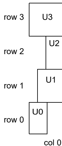
Figure 105 Right-Aligned Relative Placement Group With One Cell That is Left Aligned
