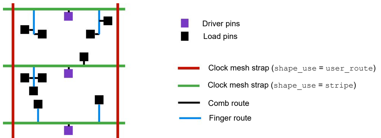
Figure 44 Fishbone Topology
