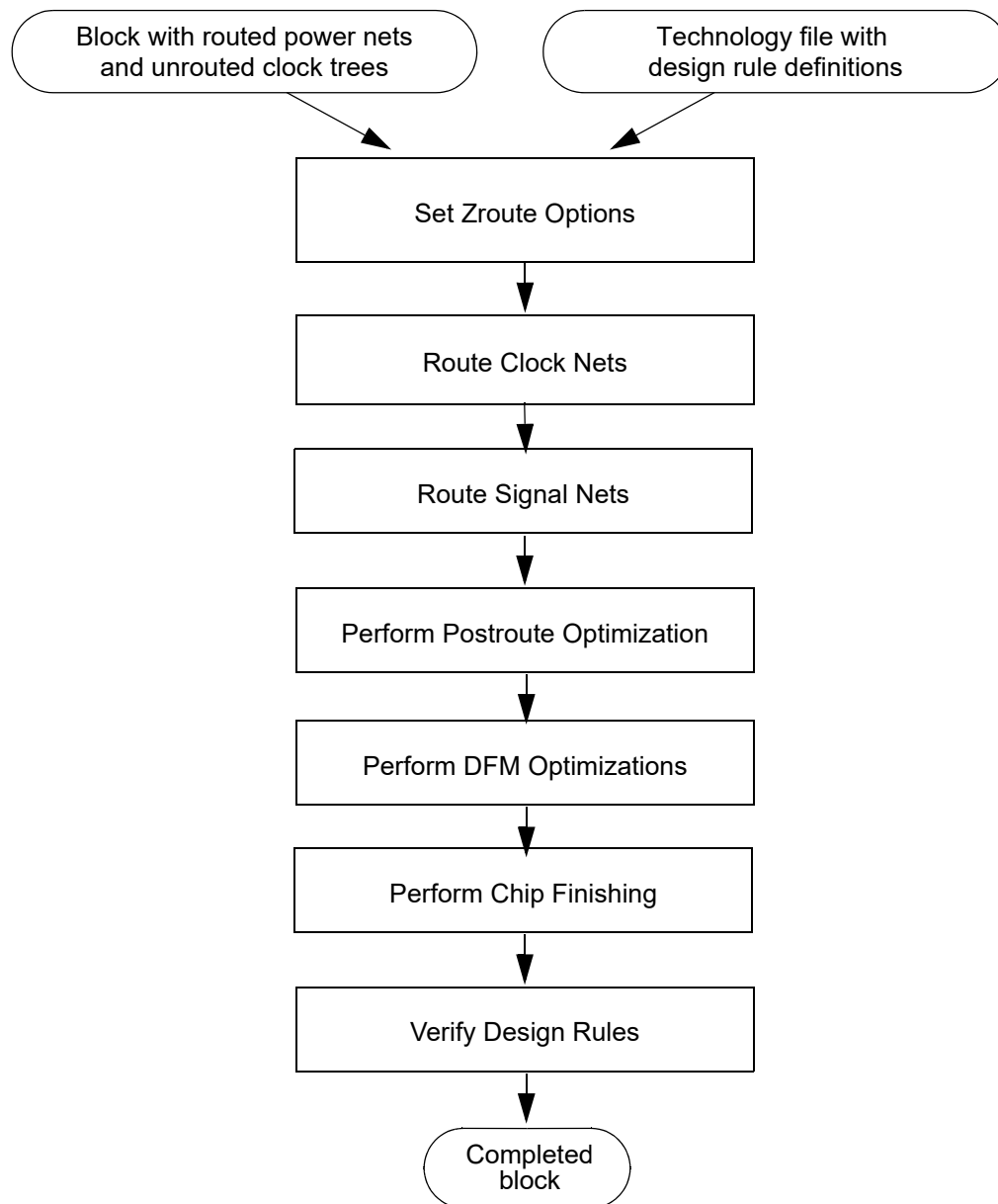
Figure 52 Basic Zroute Flow
