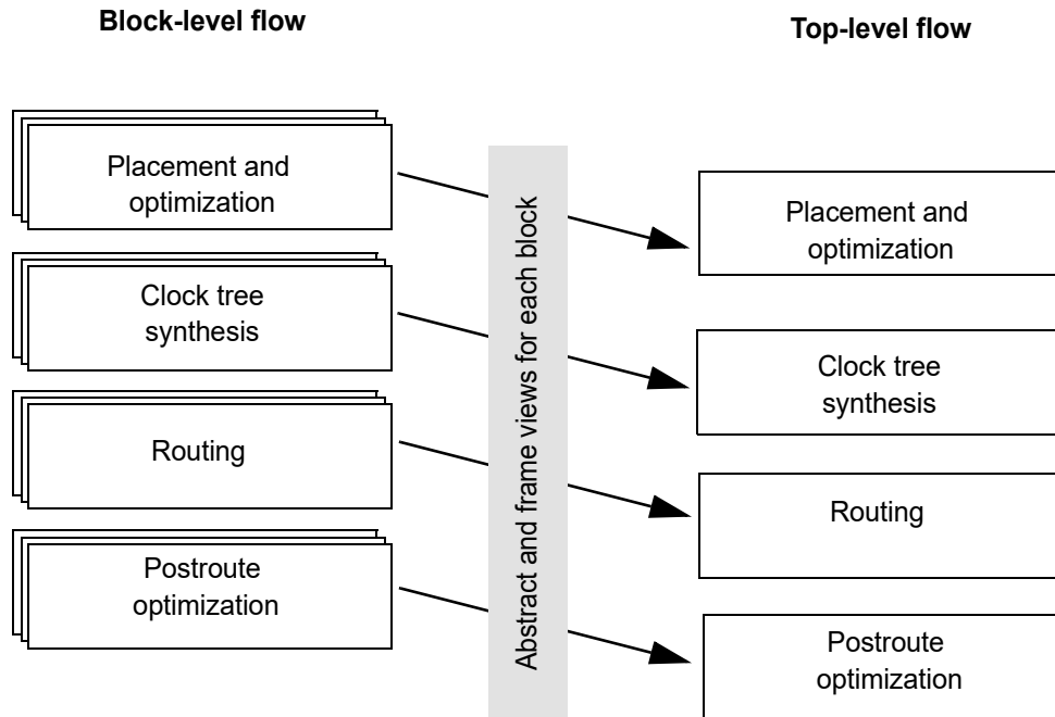
Figure 120 Top and Block Levels Implemented in Parallel
