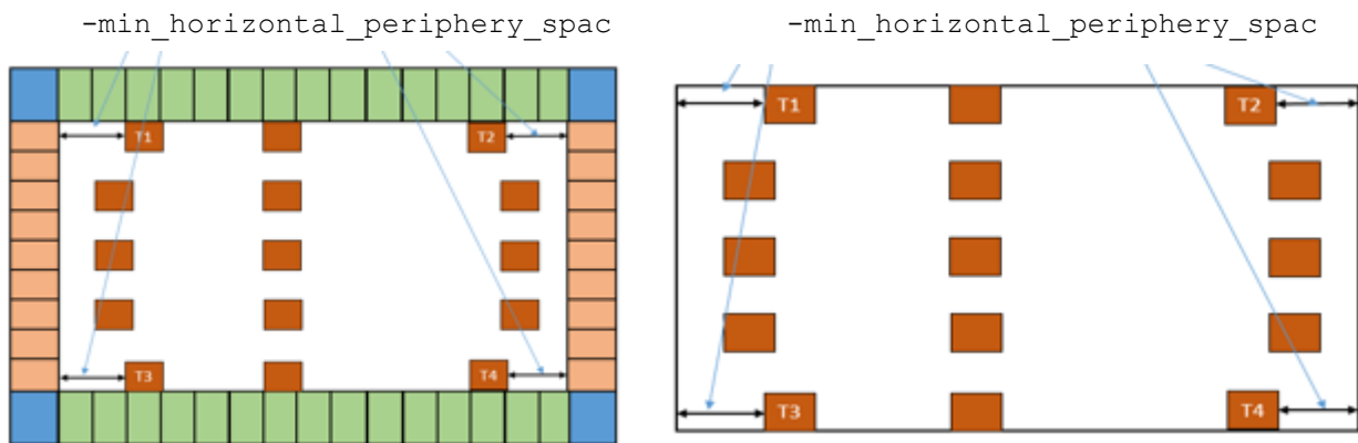
Figure 74 Tap Cell Boundary Row Spacing
