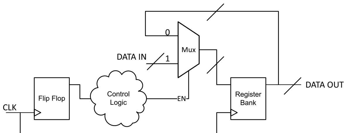
Figure 7 Synchronous Load-Enable Register With Multiplexer
